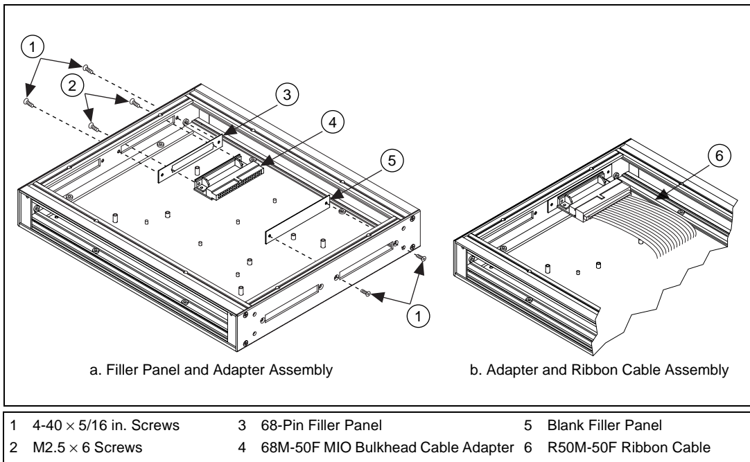
Figure 7. Installing the 68M-50F MIO Bulkhead Cable
