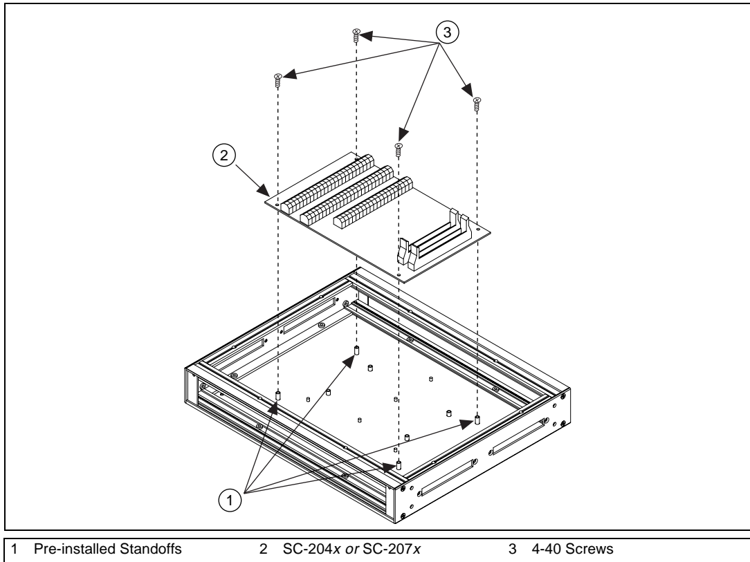
Figure 3. Installing the SC-204x or SC-207x
